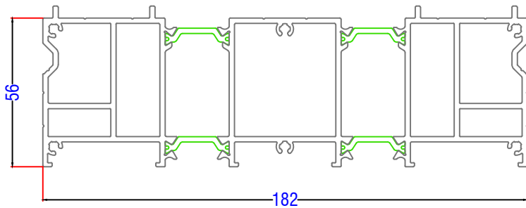
4304 - Tri Track Drainage Base
